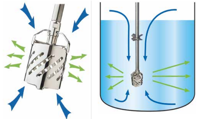
ROTOSOLVER® head for RS-02
